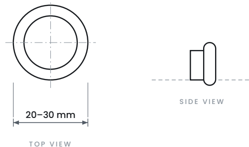
TECHNICAL DRAWING
